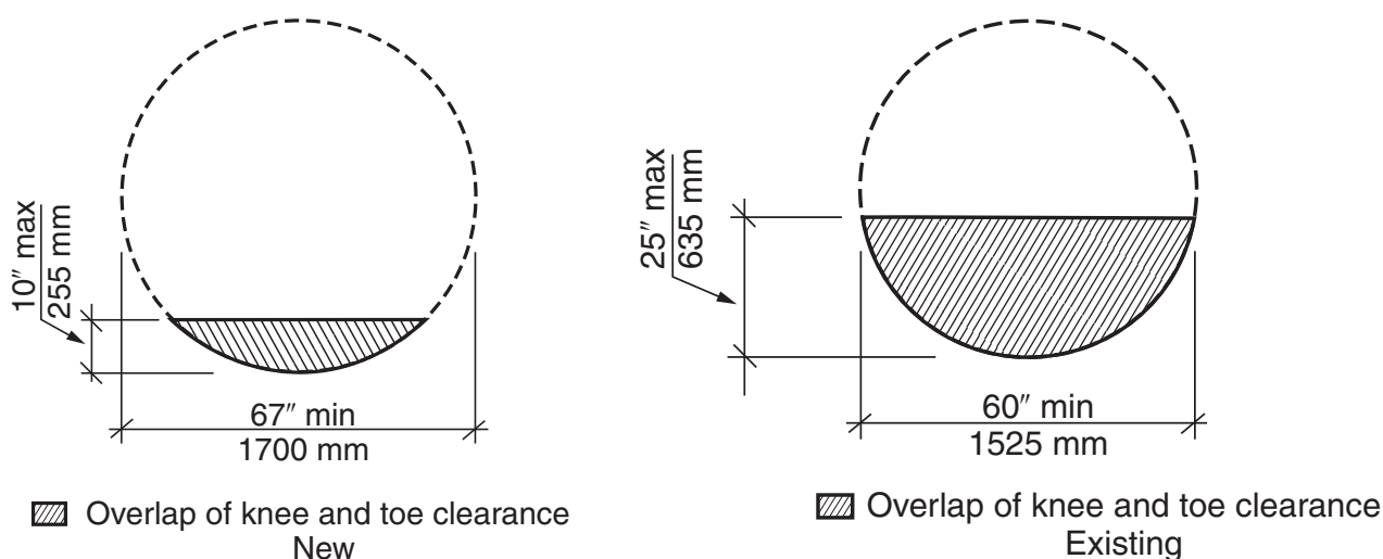
Commentary Figure 301.5 COMPARISON OF TURNING SPACE REQUIREMENTS FOR NEW AND EXISTING BUILDINGS
