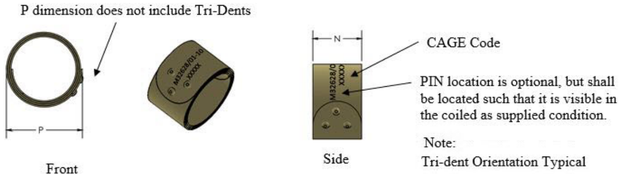
FIGURE 1. Tri-Dent splice configuration (M32628/01-10).
